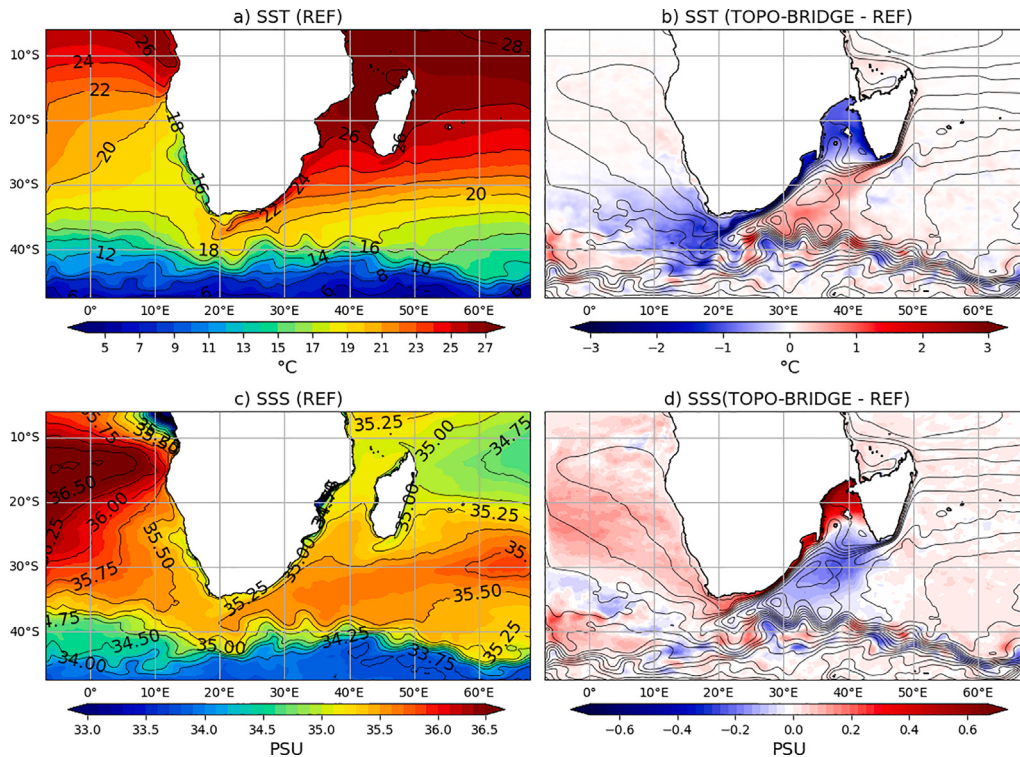
Fig. 8. (a) SST and (c) SSS averaged over 2008–2017 for the reference experiment (respectively CI = 2 ^{\circ}\text{C} and CI = 0.25 PSU). (b) SST and (d) SSS difference between the experiment with modified bathymetry and the reference experiment averaged over 2008–2017, contours indicate the mean SSH (CI = 10 cm).
