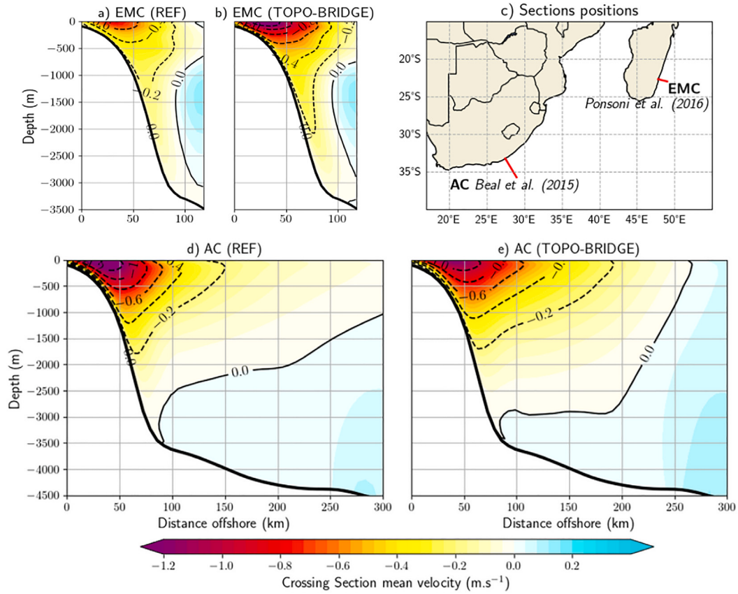
Fig. 7. Mean velocities orthogonal to the EMC and AC sections defined by Ponsoni et al. (2016) and Beal et al. (2015) averaged over 2008–2017, for the REF (left) and for TOPO-BRIDGE (right). (CI 20 \text{cm s}^{-1} , solid northward, dashed southward).
