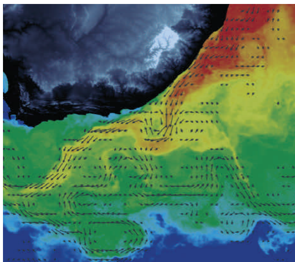
Sea surface temperatures measurements of the Agulhas Current from SEVIRI overlaid with geostrophic currents derived from altimetry measurements of the sea level. Courtesy: Marjolaine Krug (CSIR - Earth Observation).
